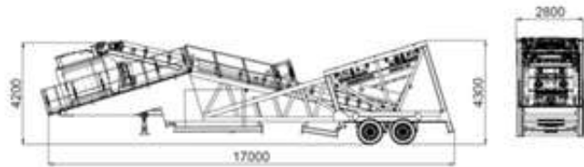
TRANSPORT POSITION
